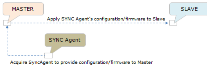
Graphics 5: Master asks SyncAgent to provide configuration/firmware, and then apply to Slave
