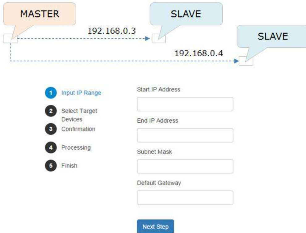
Graphics 3: IP Range Assignment
