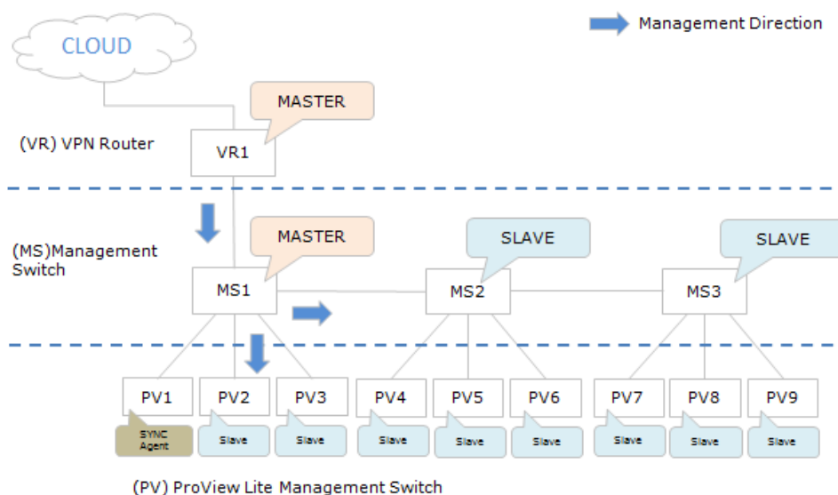
Graphics 1: IXM Topology
